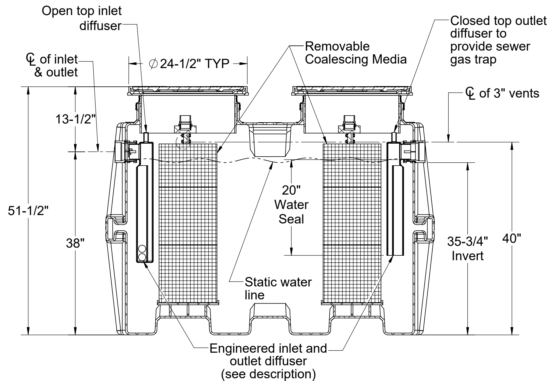
SECTION "A-A"
