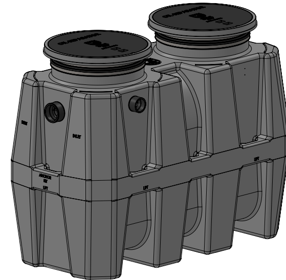
OS-100 OS SERIES 100 GPM High Efficiency Oil/Water Separator
