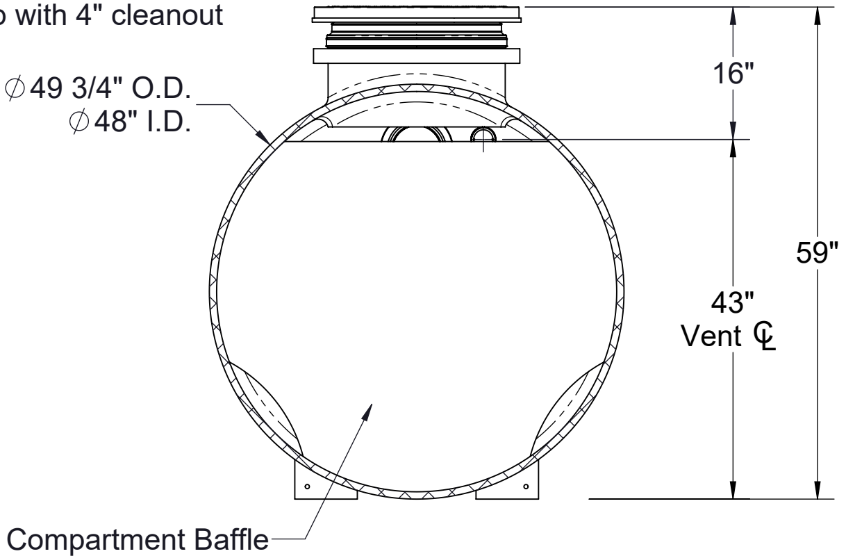
SECTION B-B
