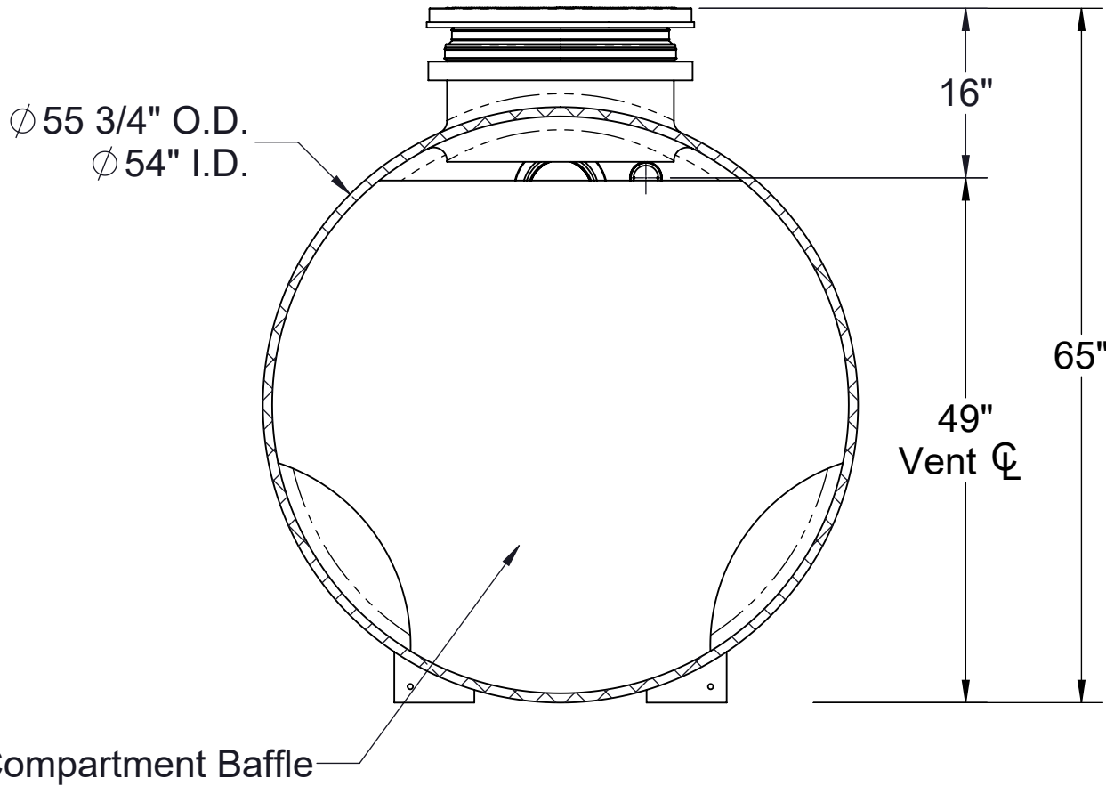
SECTION B-B
