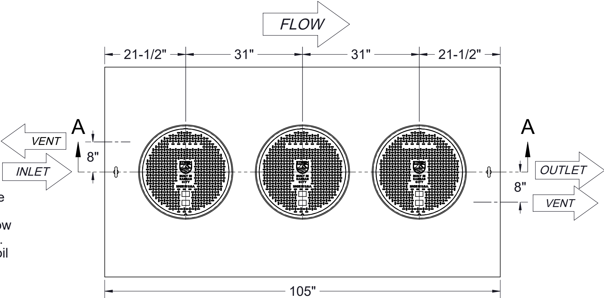
TOP VIEW
