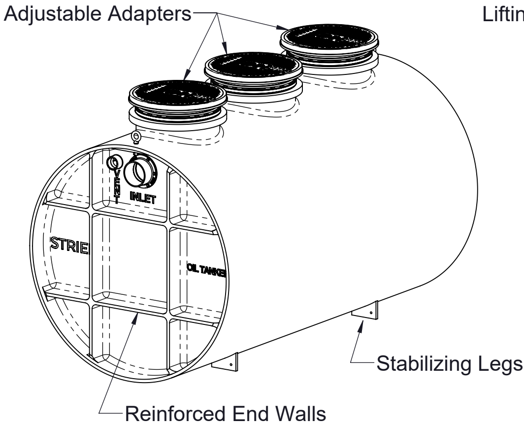
ISOMETRIC VIEW
