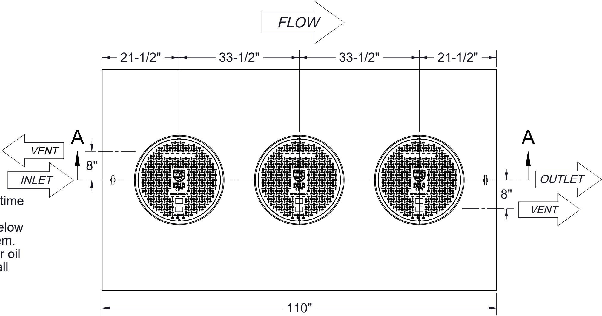
TOP VIEW
