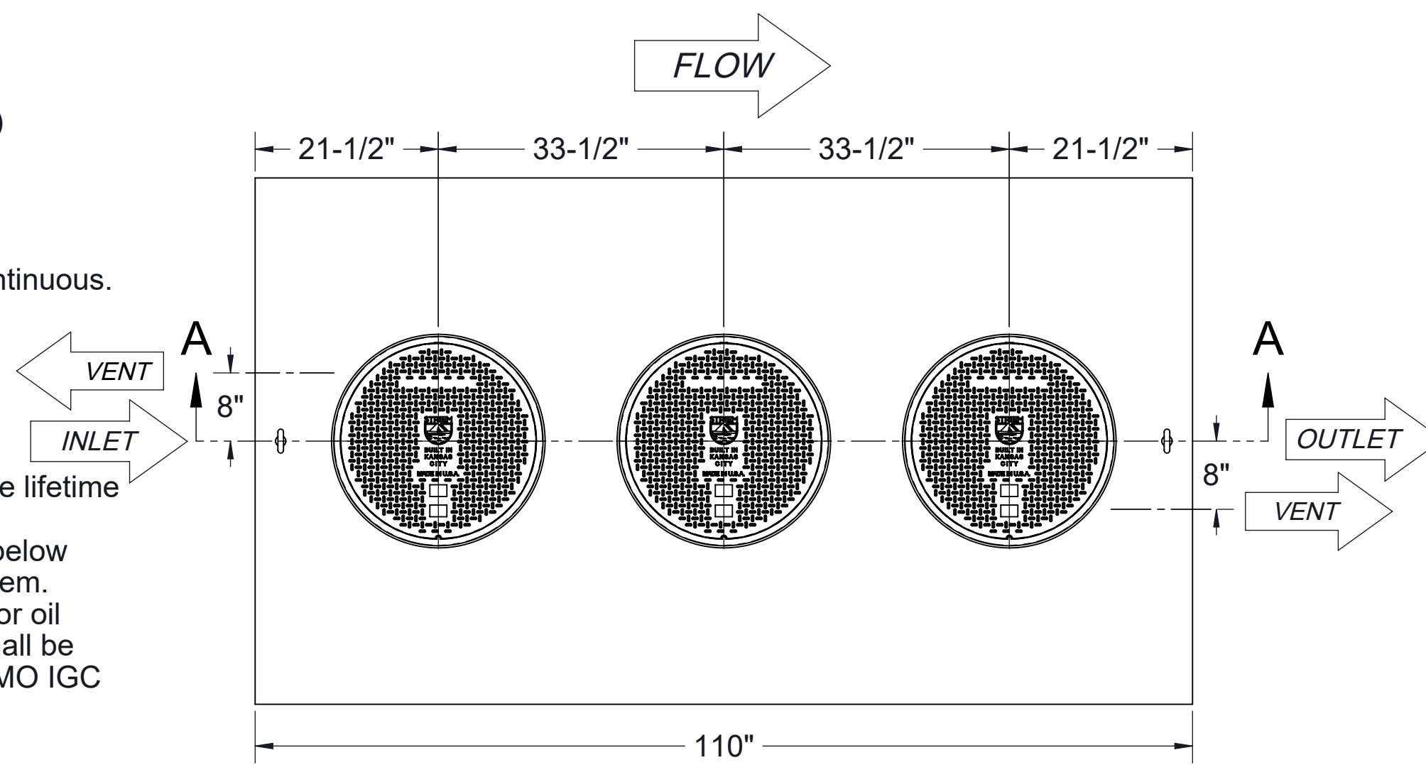
TOP VIEW
