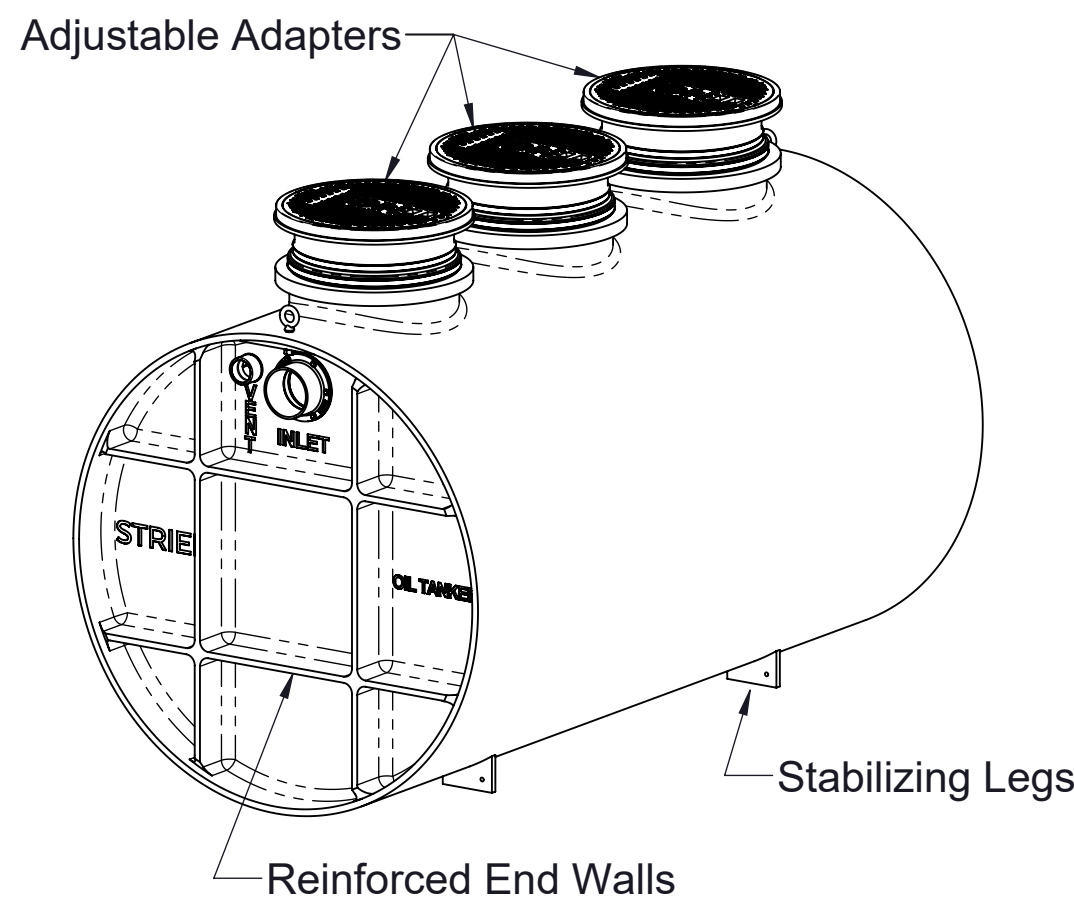
ISOMETRIC VIEW
