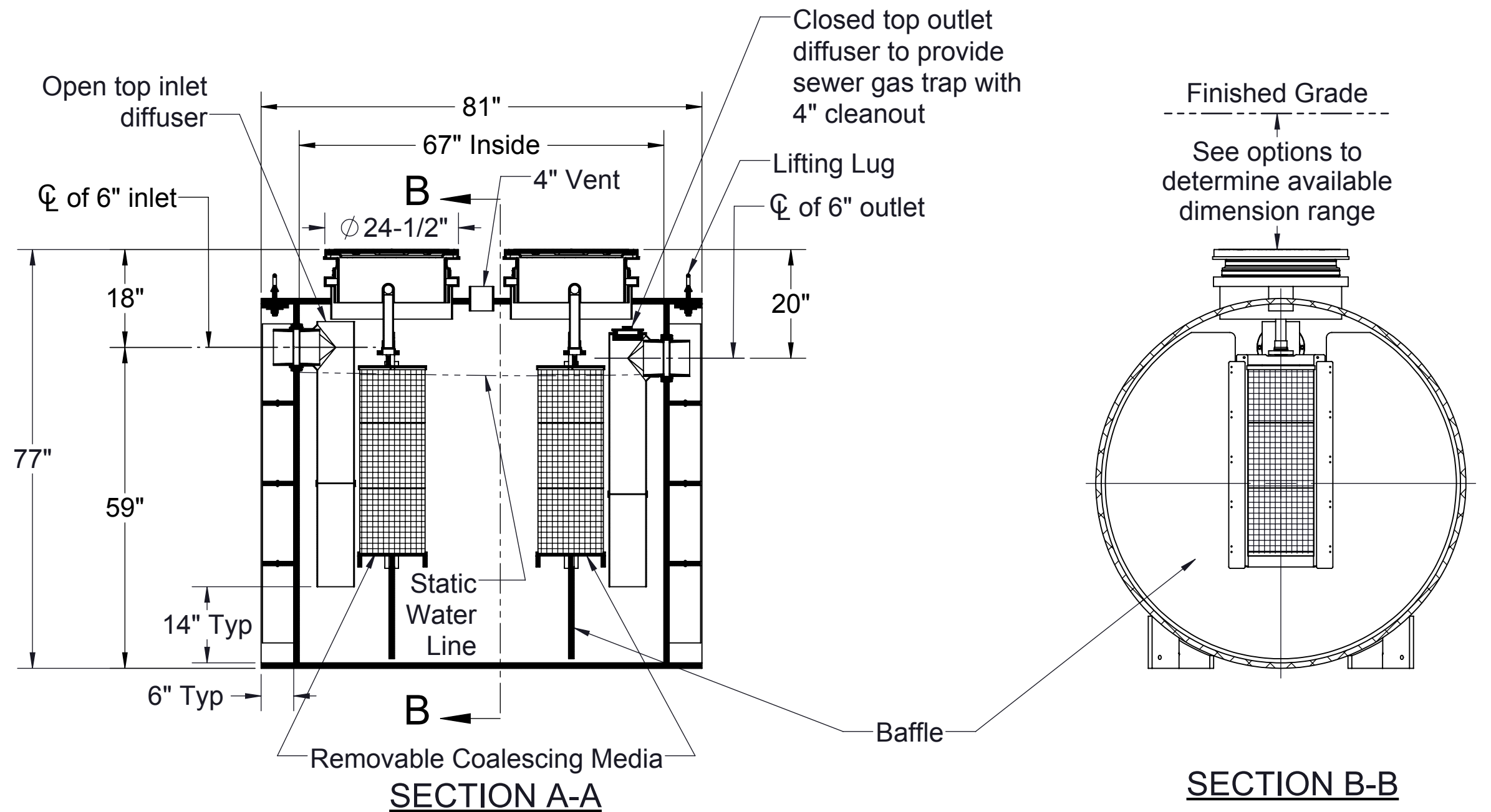
ISOMETRIC VIEW
