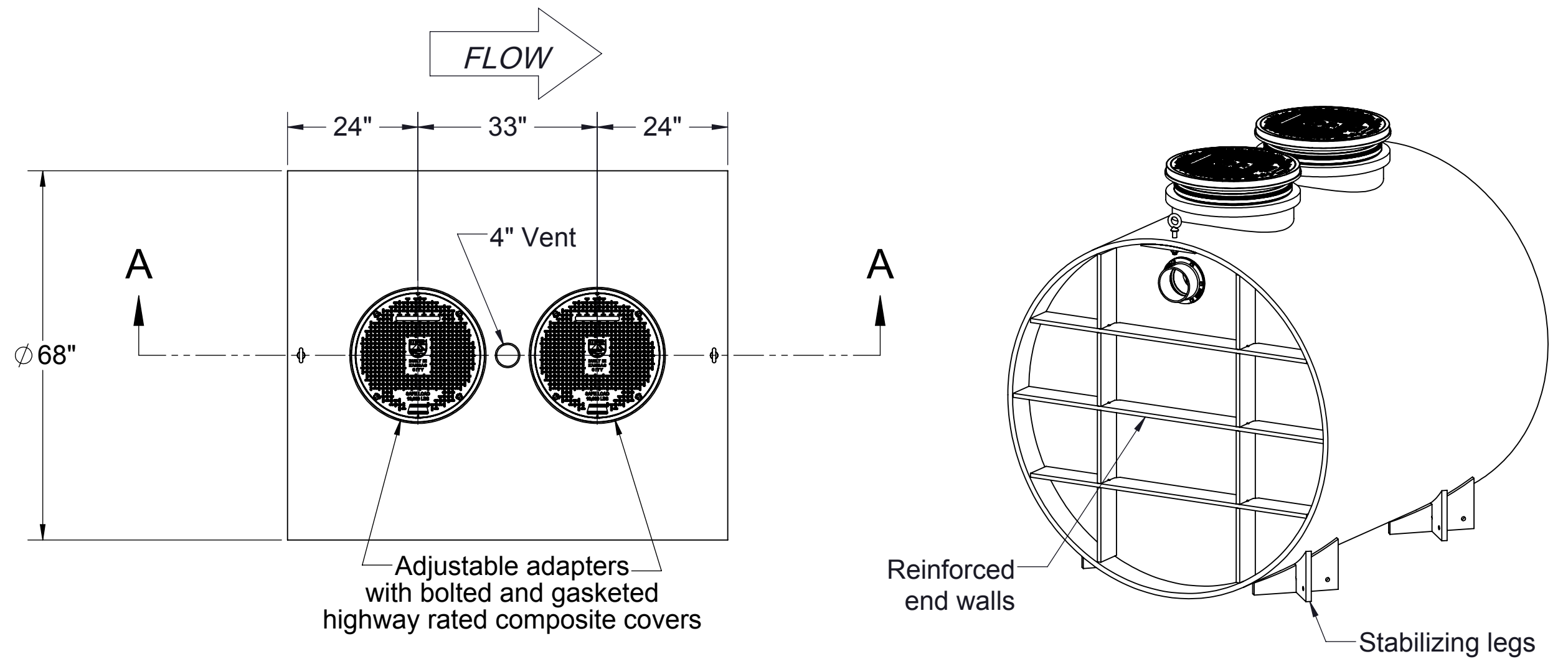
TOP VIEW
