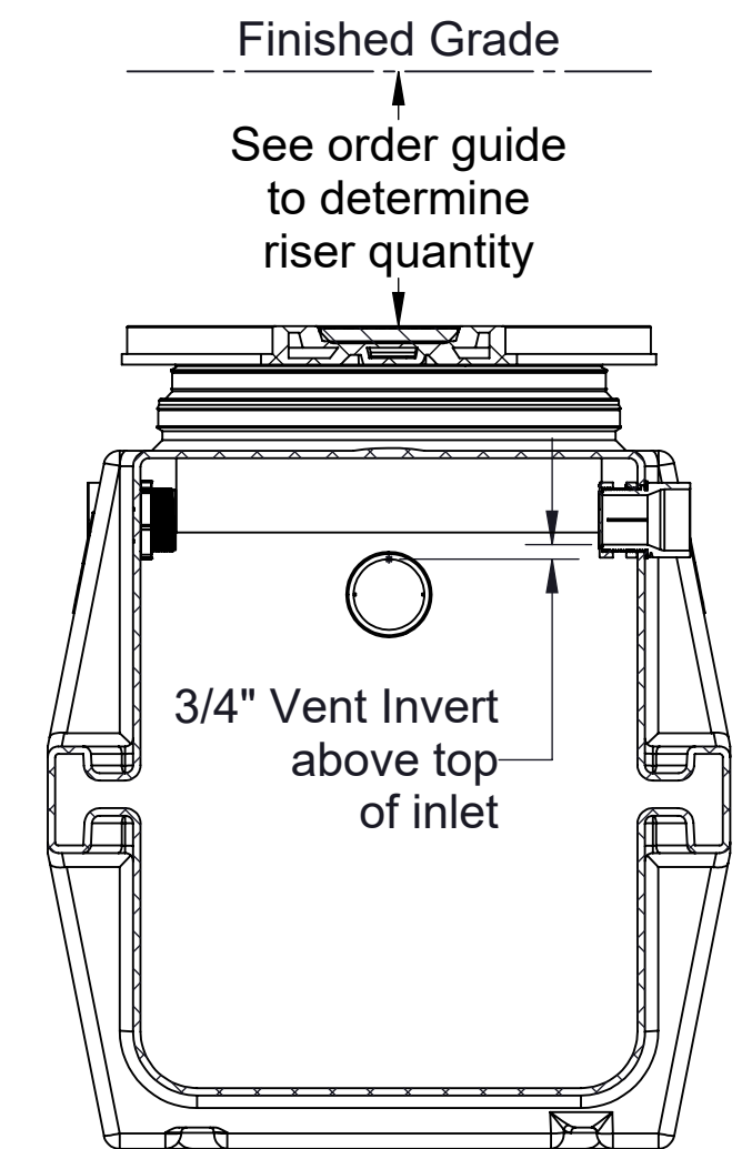
SECTION B-B
