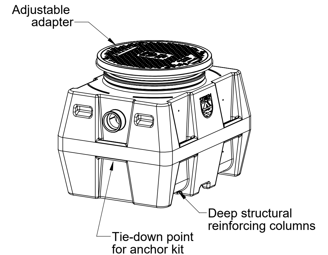
ISOMETRIC VIEW
