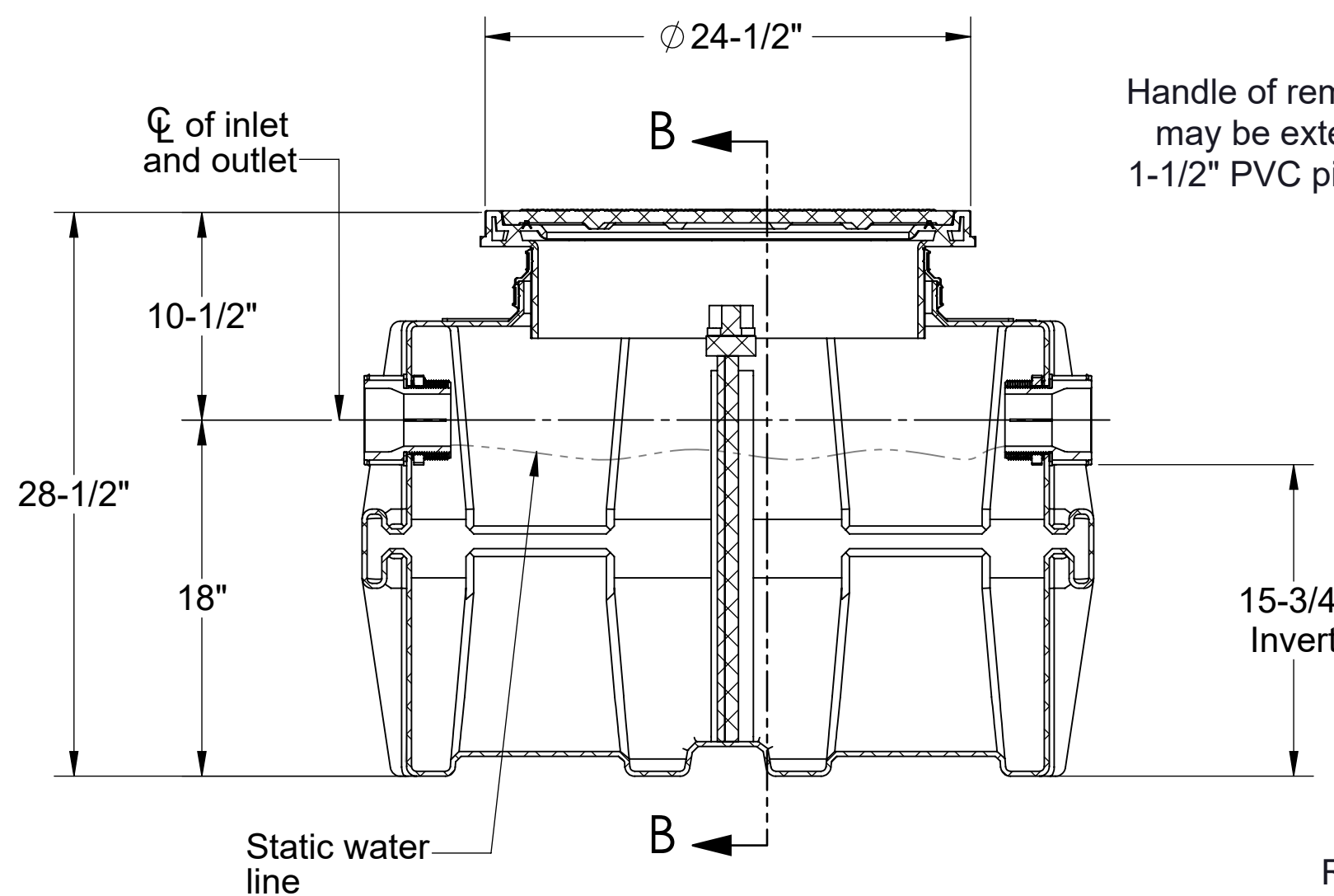
SECTION "A-A"
