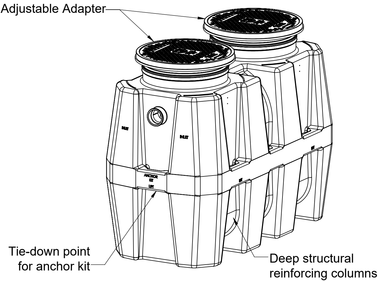
ISOMETRIC VIEW
