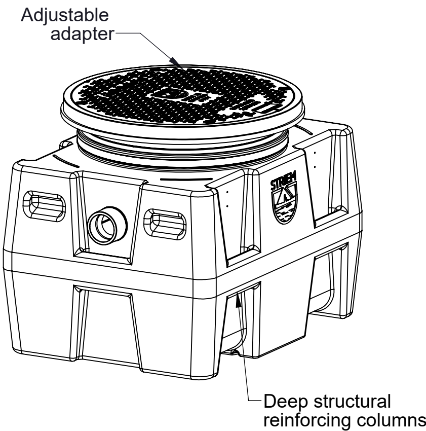
ISOMETRIC VIEW
