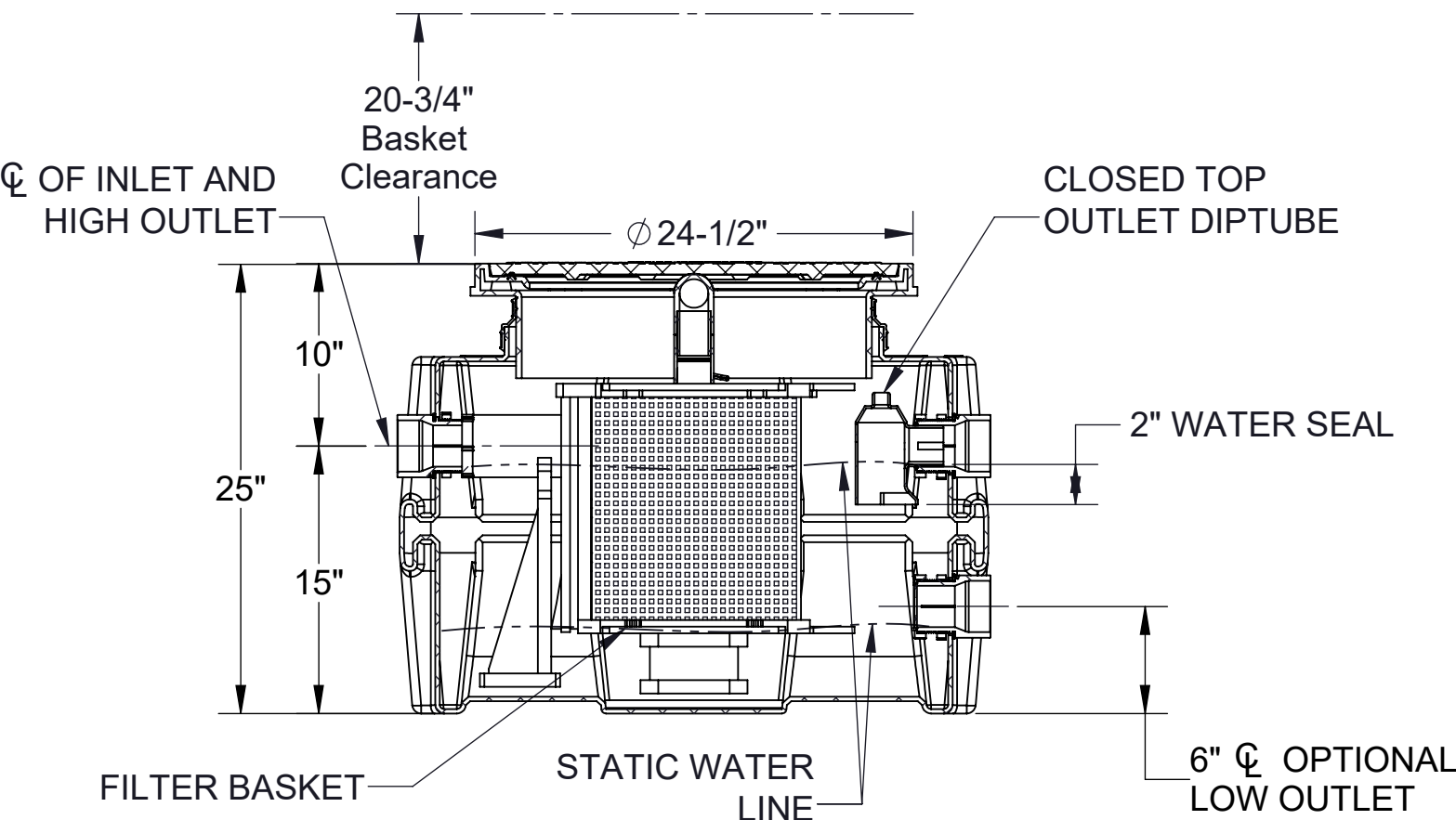
SECTION "A-A"
