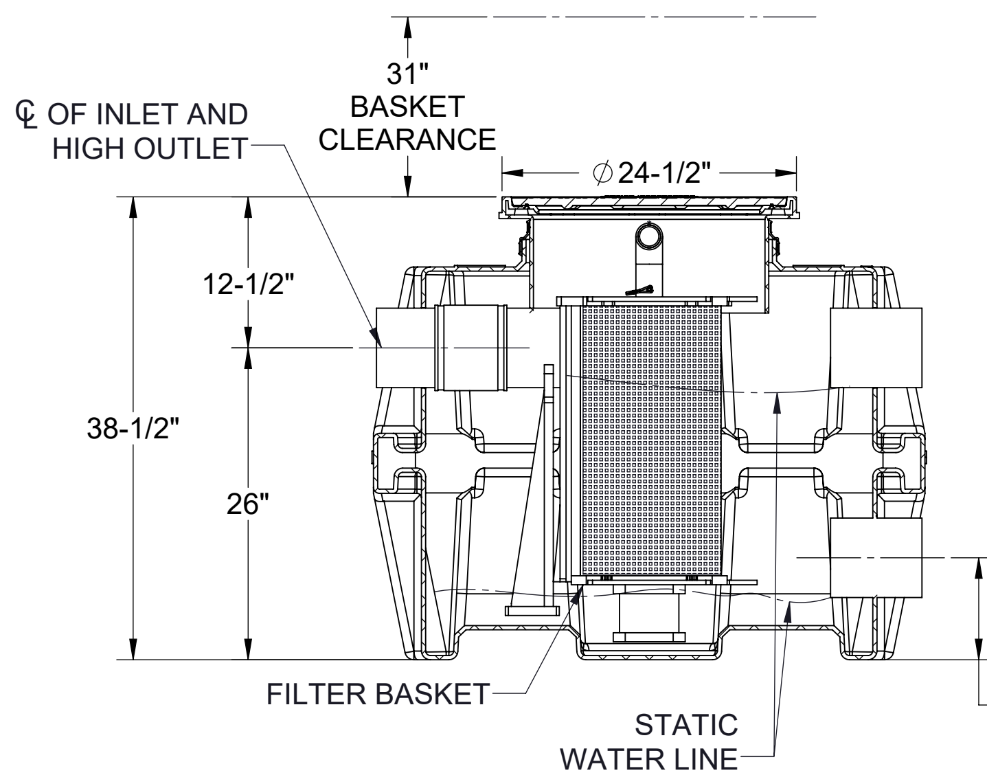
SECTION "A-A"
