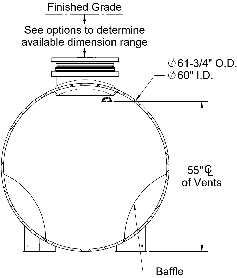
SECTION B-B
