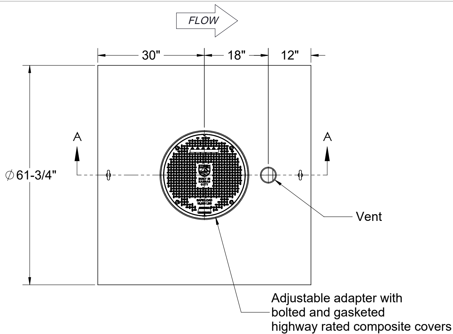
TOP VIEW
