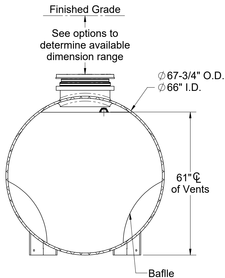
SECTION B-B
