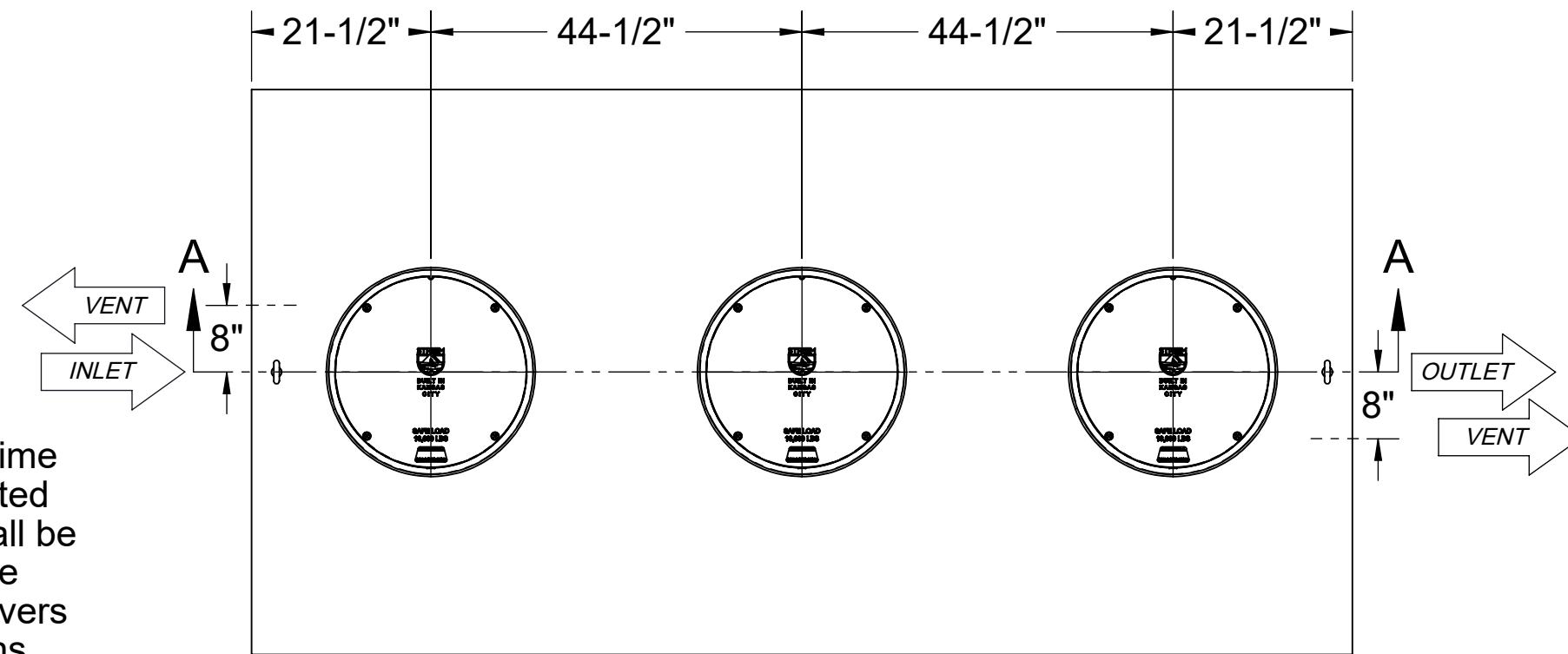
TOP VIEW
