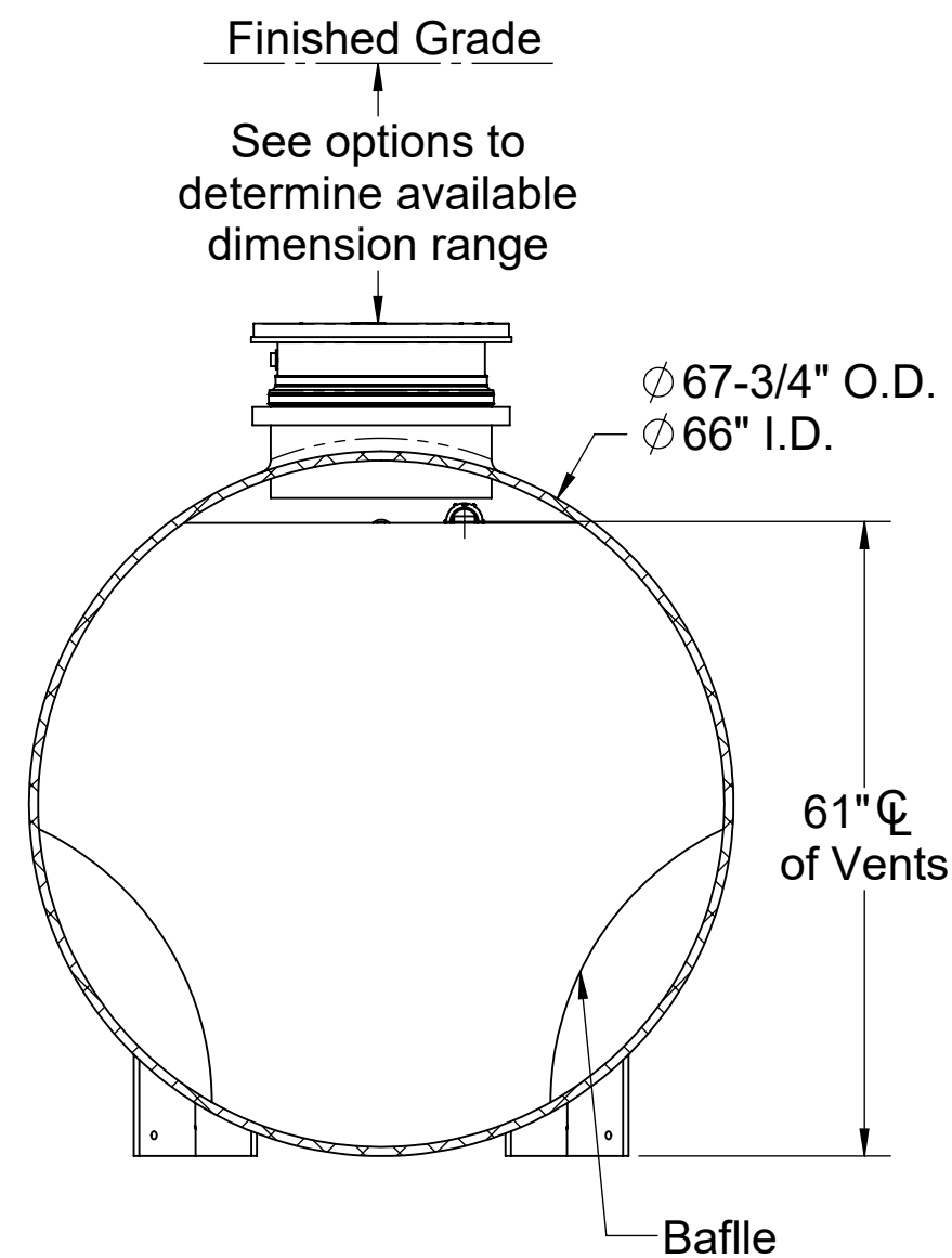
SECTION B-B
