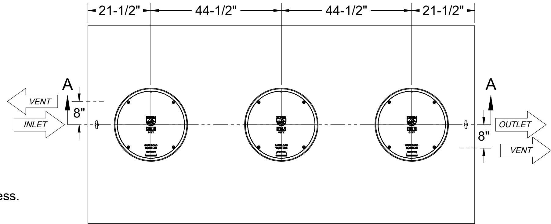
TOP VIEW
