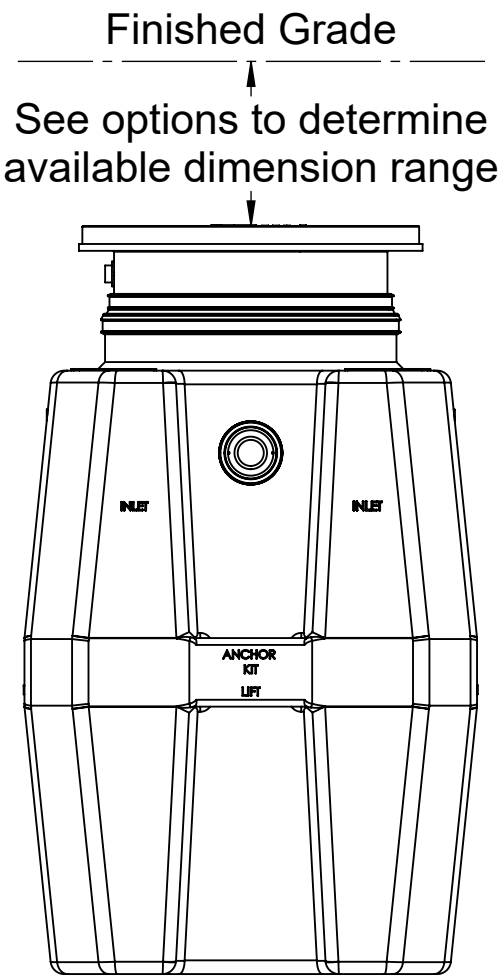
END VIEW
