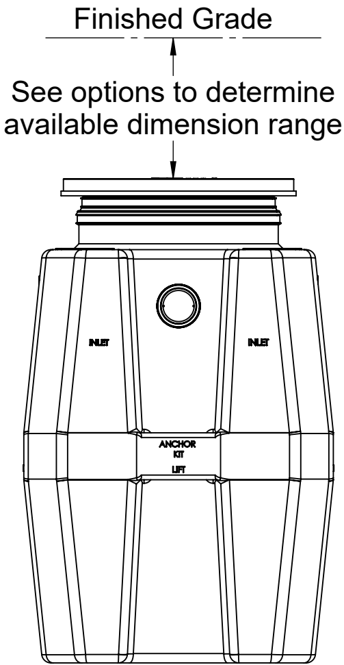
END VIEW
