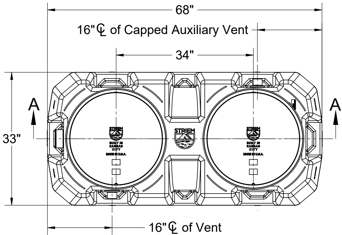
TOP VIEW
