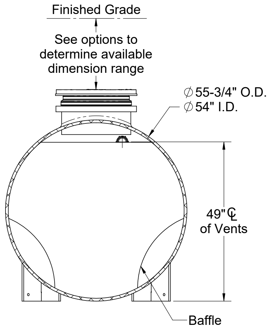
SECTION B-B
