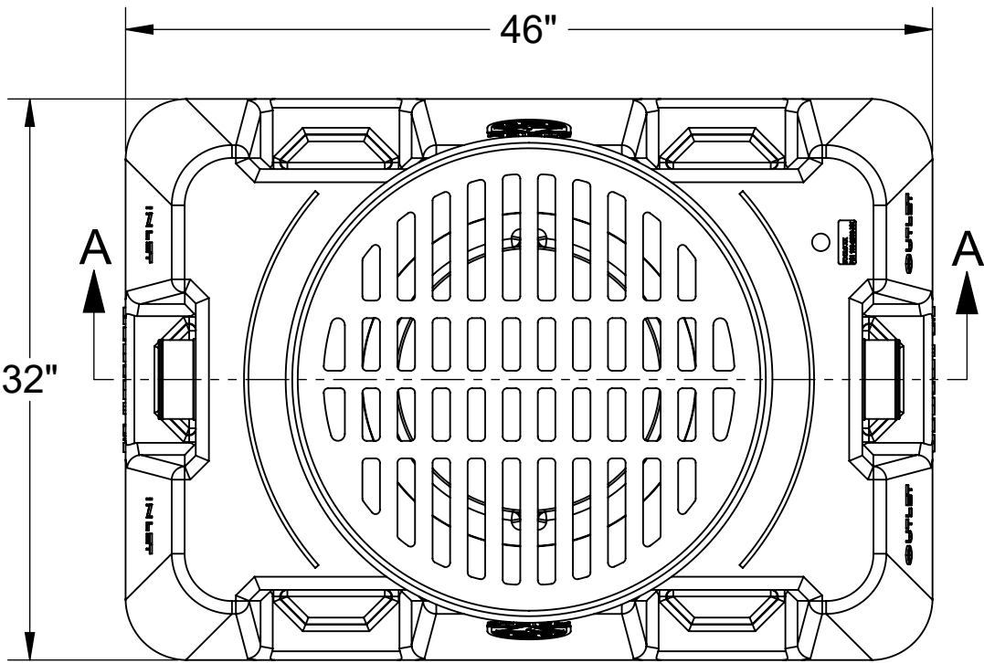
TOP VIEW
