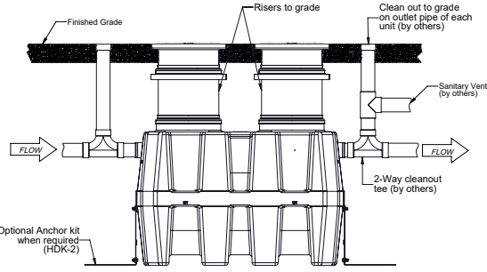
SIDE VIEW DETAIL
