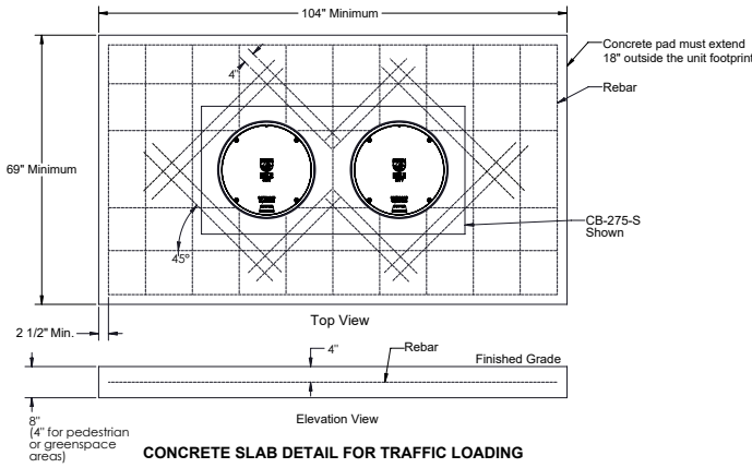
CONCRETE SLAB DETAIL FOR TRAFFIC LOADING
