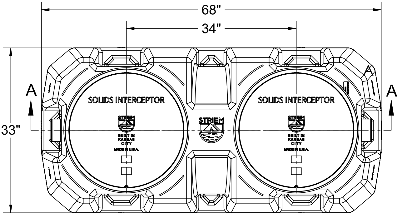
TOP VIEW
