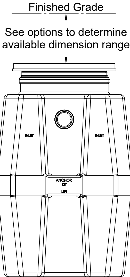
END VIEW
