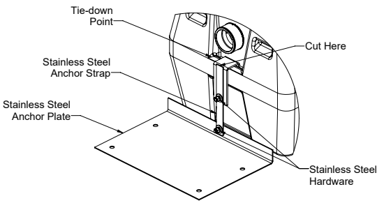
HIGH WATER ANCHOR KIT INSTALLATION DETAIL (HDK-2)
