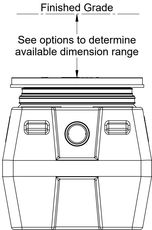
END VIEW
