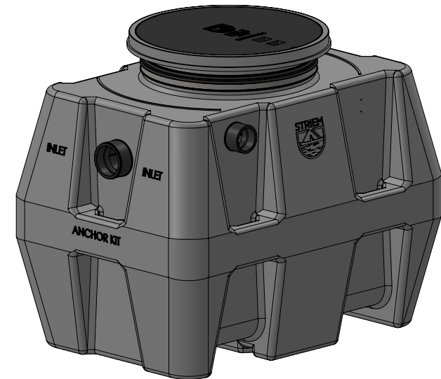
FLI-125 FLAMMABLE LIQUID INTERCEPTOR 125 GAL
