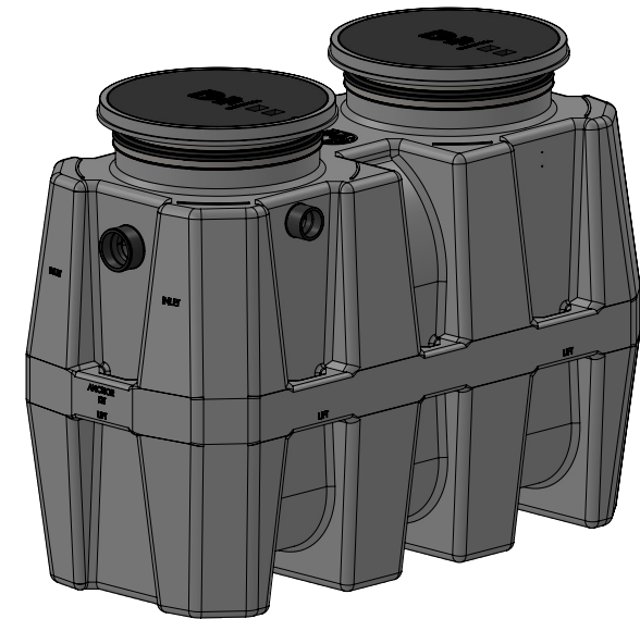
FLI-275 FLAMMABLE LIQUID INTERCEPTOR 250 GAL
