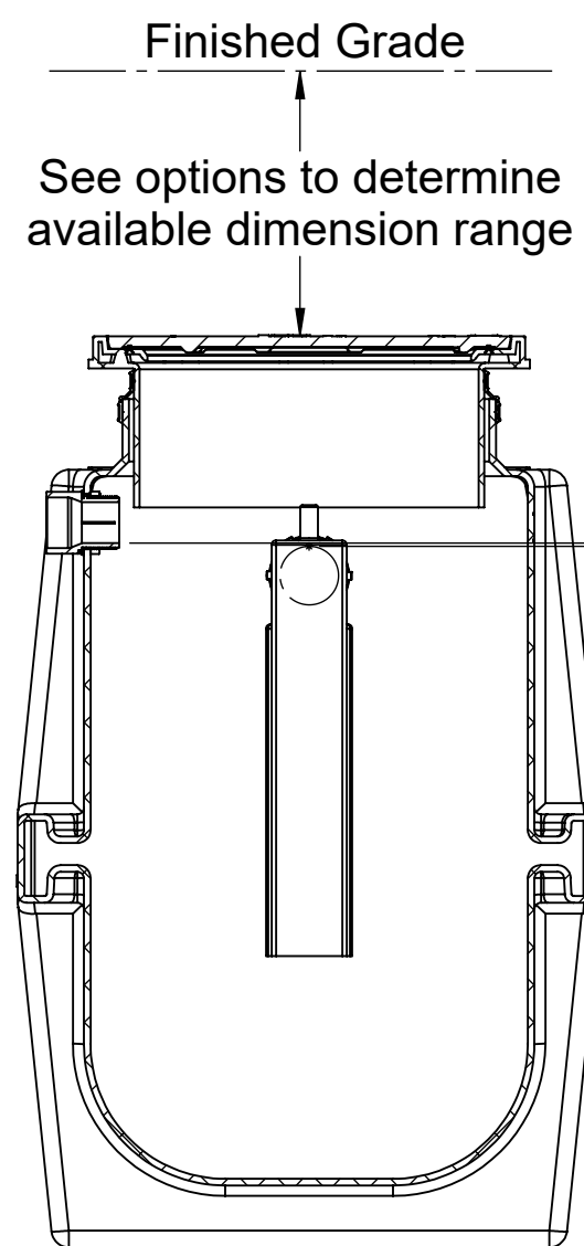
SECTION B-B
