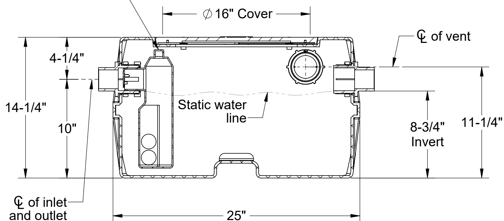
SECTION "A-A"
