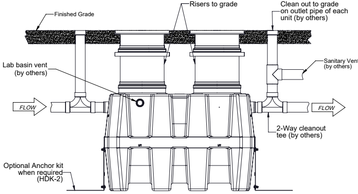
SIDE VIEW DETAIL
