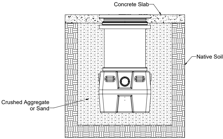
EXCAVATION AND BACKFILL DETAIL (INTERIOR OR EXTERIOR)
