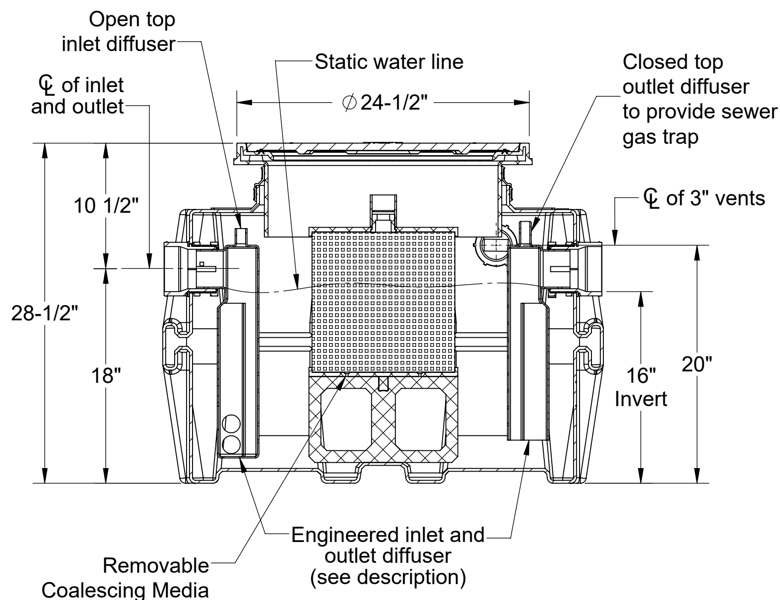
SECTION "A-A"
