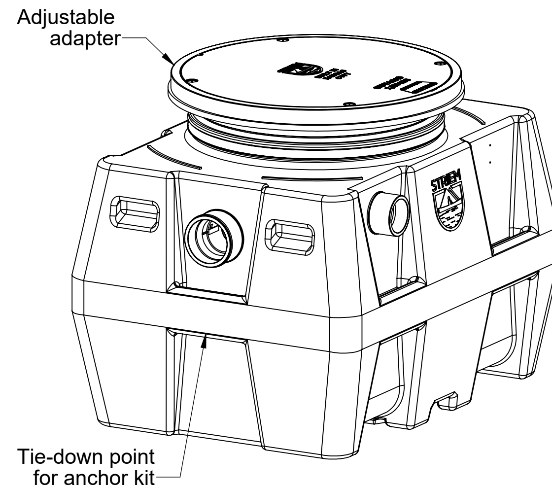
ISOMETRIC VIEW
