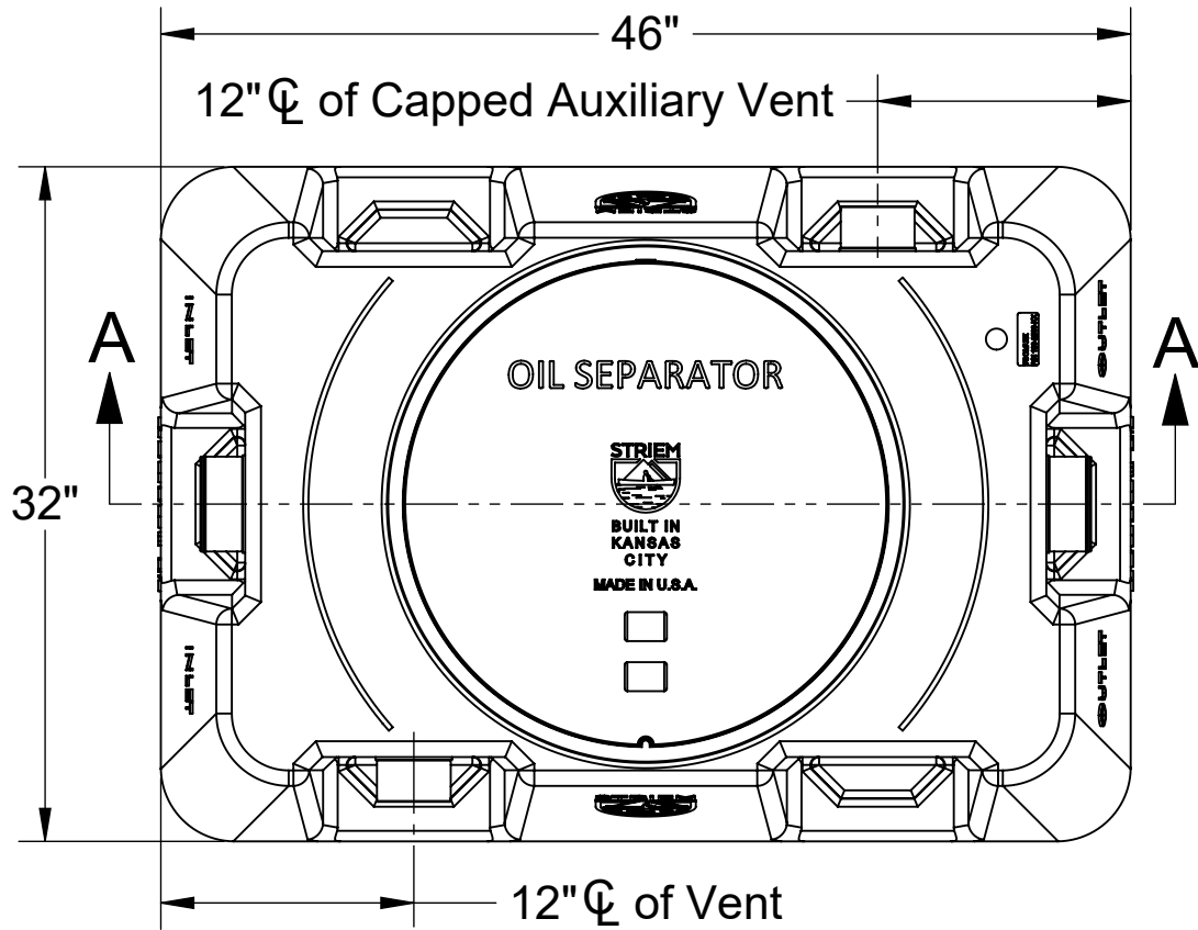
TOP VIEW
