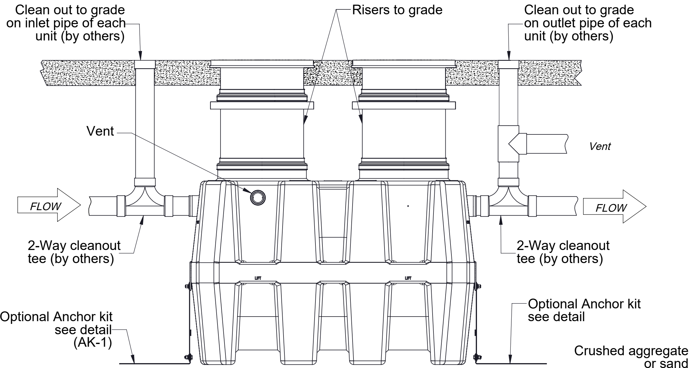
SIDE VIEW DETAIL
