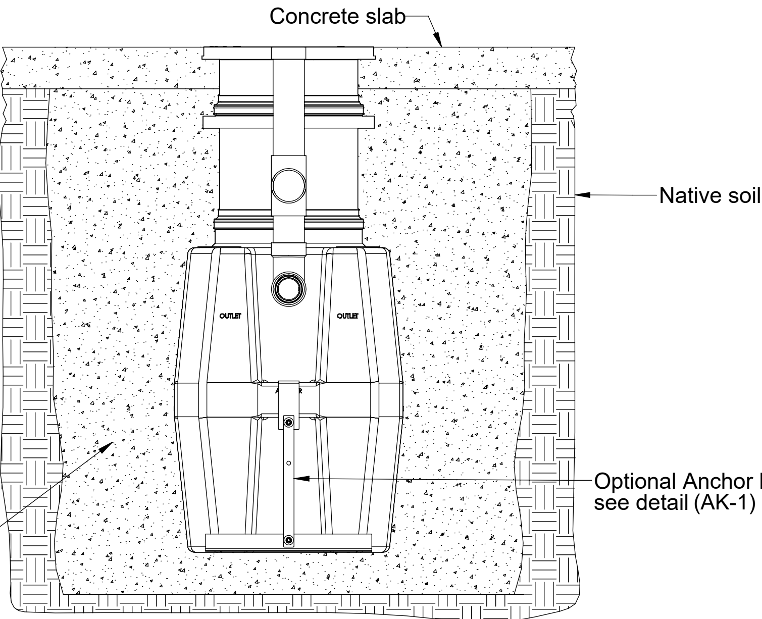
EXCAVATION AND BACKFILL DETAIL (INTERIOR OR EXTERIOR)
