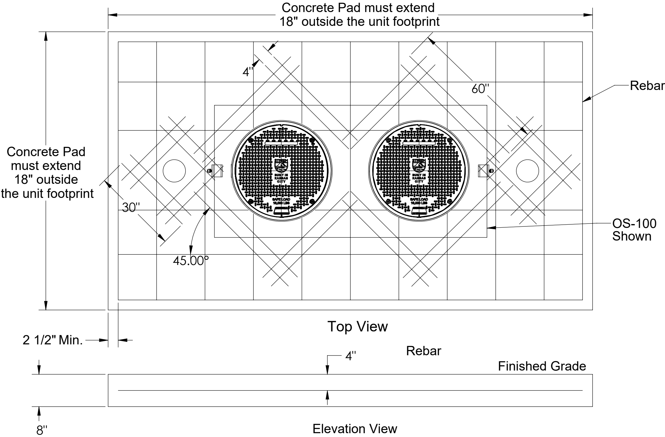
CONCRETE SLAB DETAIL FOR TRAFFIC LOADING (INTERIOR OR EXTERIOR) (OS-100 Shown)
