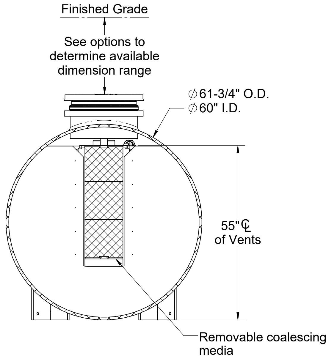
SECTION B-B
