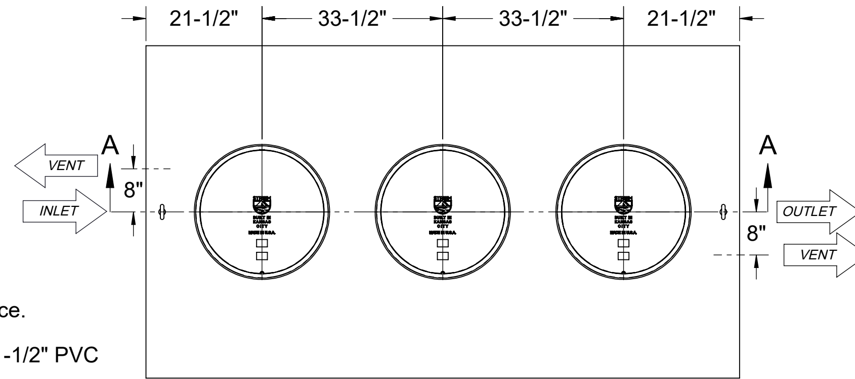
TOP VIEW
