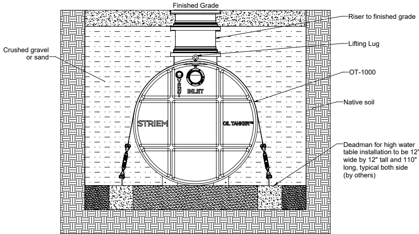
EXCAVATION AND BACKFILL DETAIL
