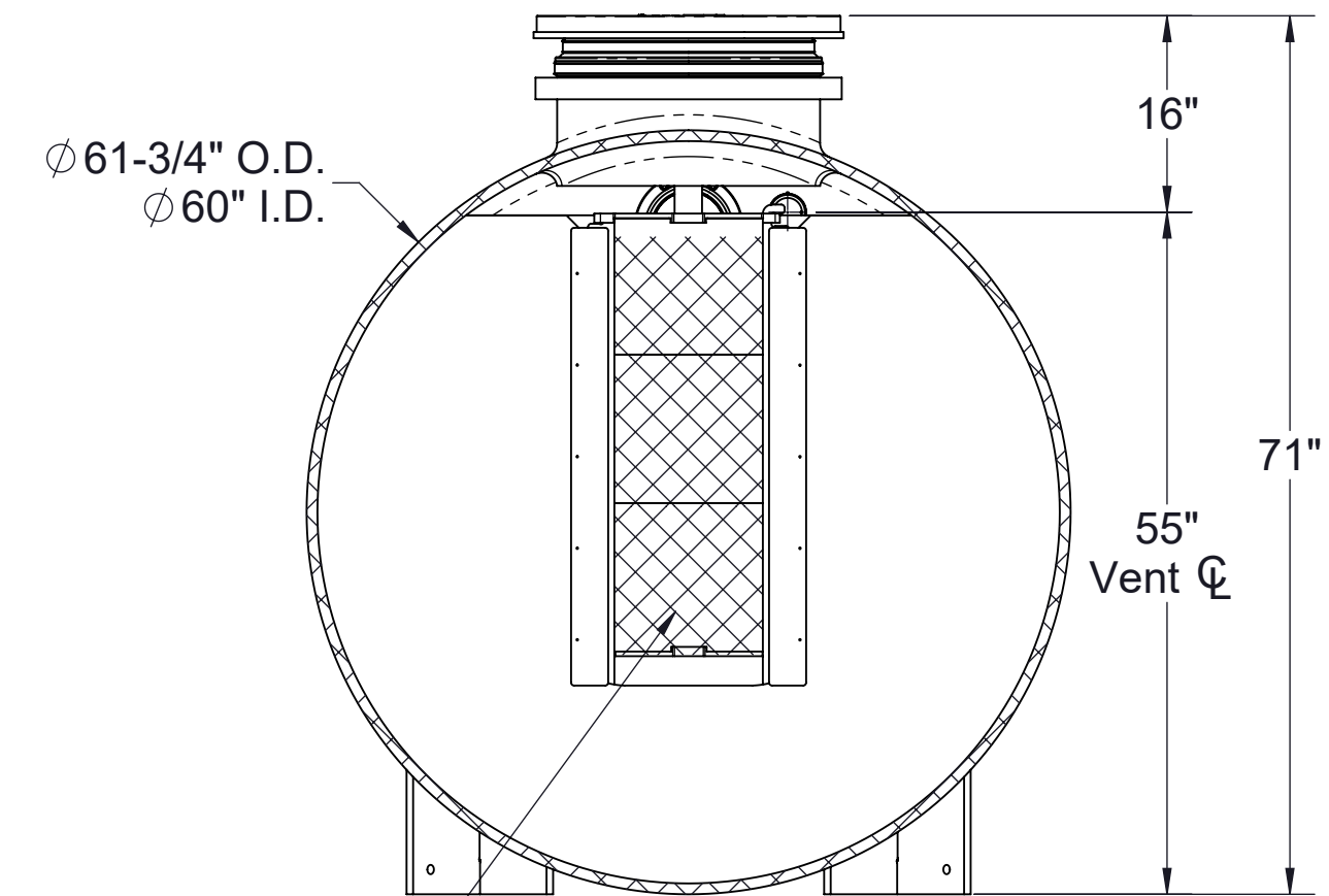
SECTION B-B
