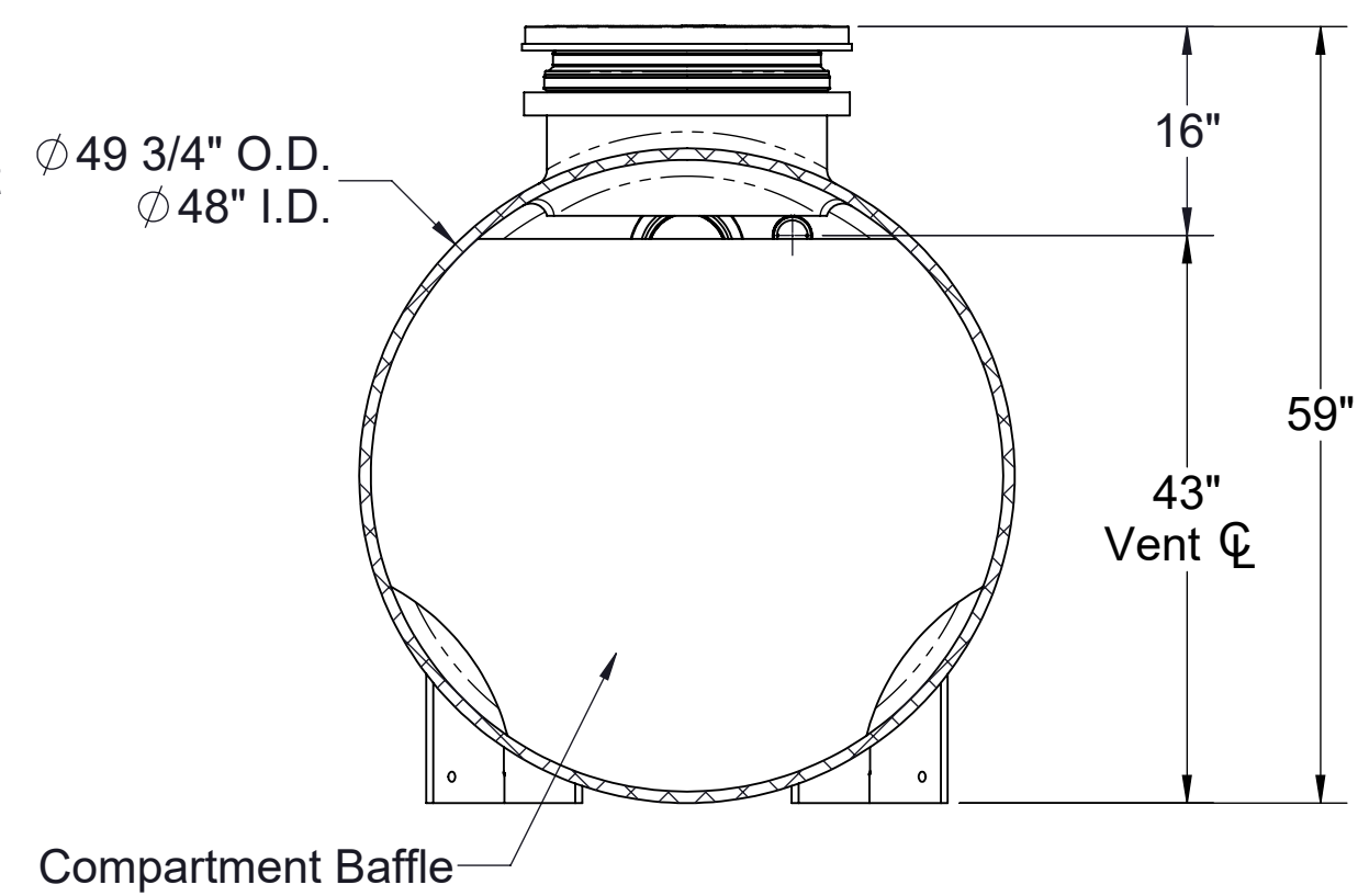
SECTION B-B
