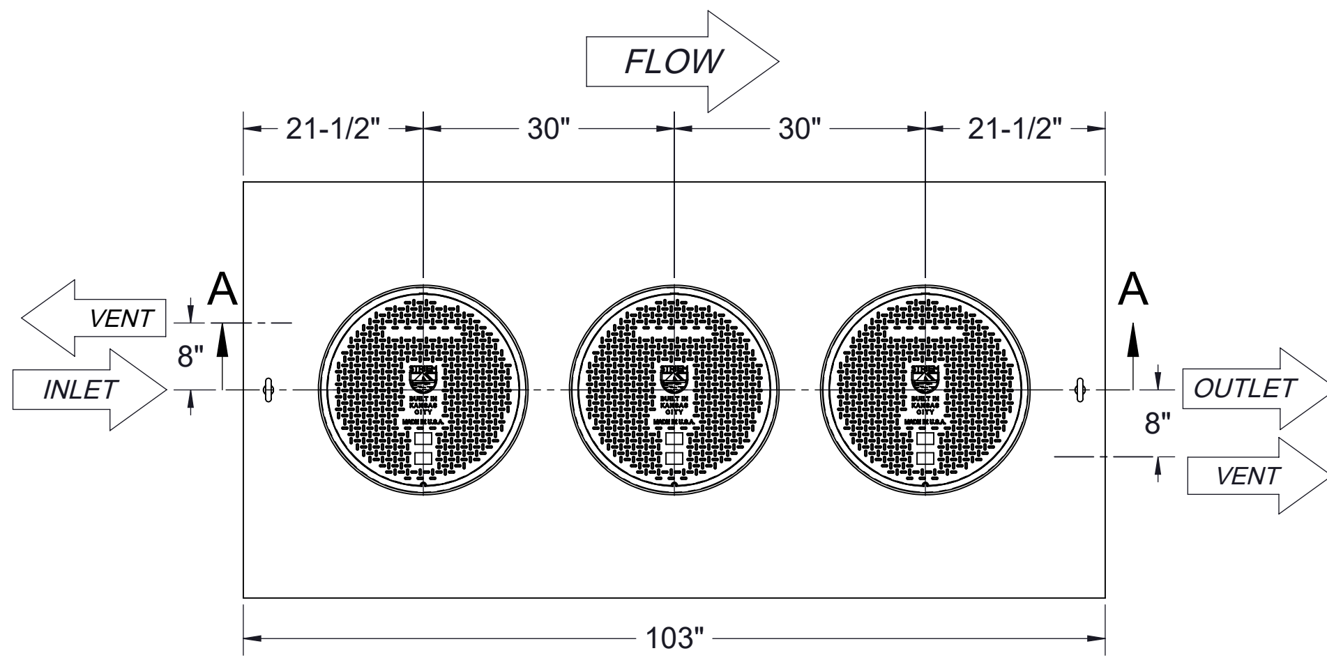
TOP VIEW
