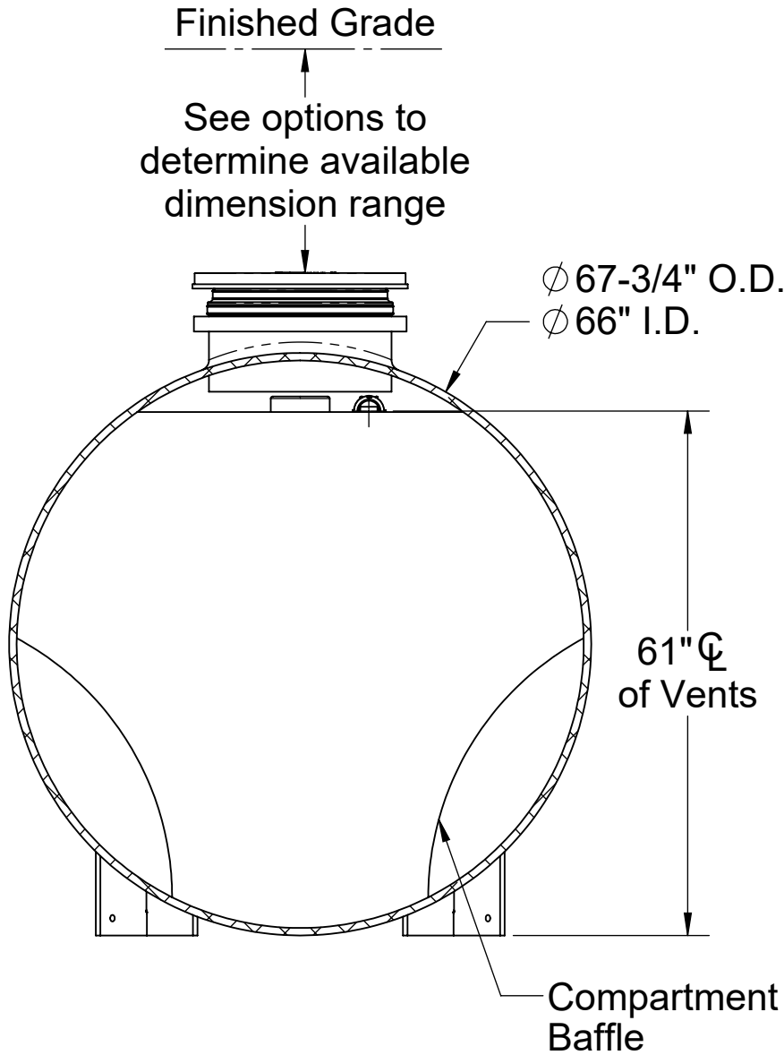
SECTION B-B
