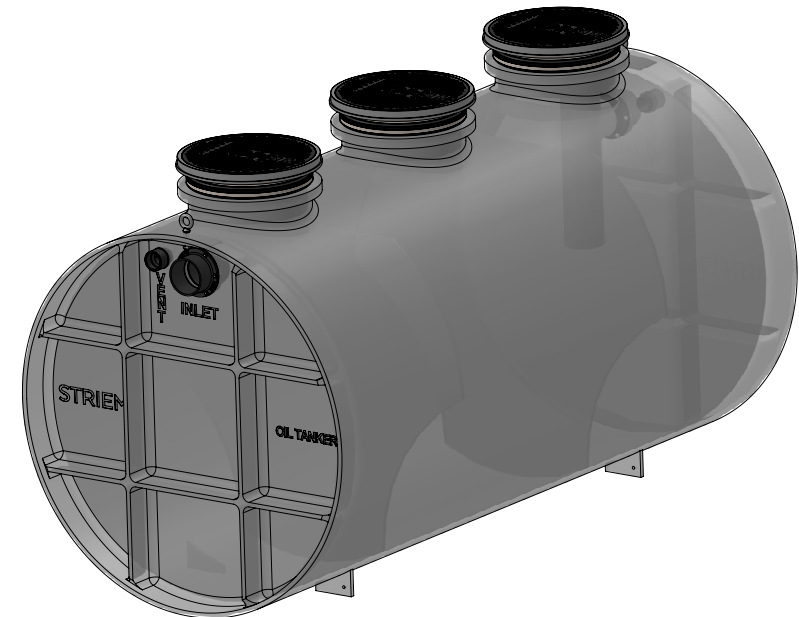
OT-1500 OIL TANKER™ SERIES 1,500 GALLON OIL SEPARATOR
