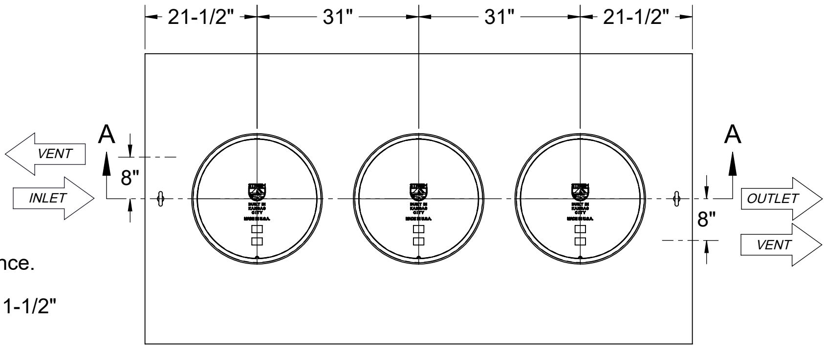
TOP VIEW
