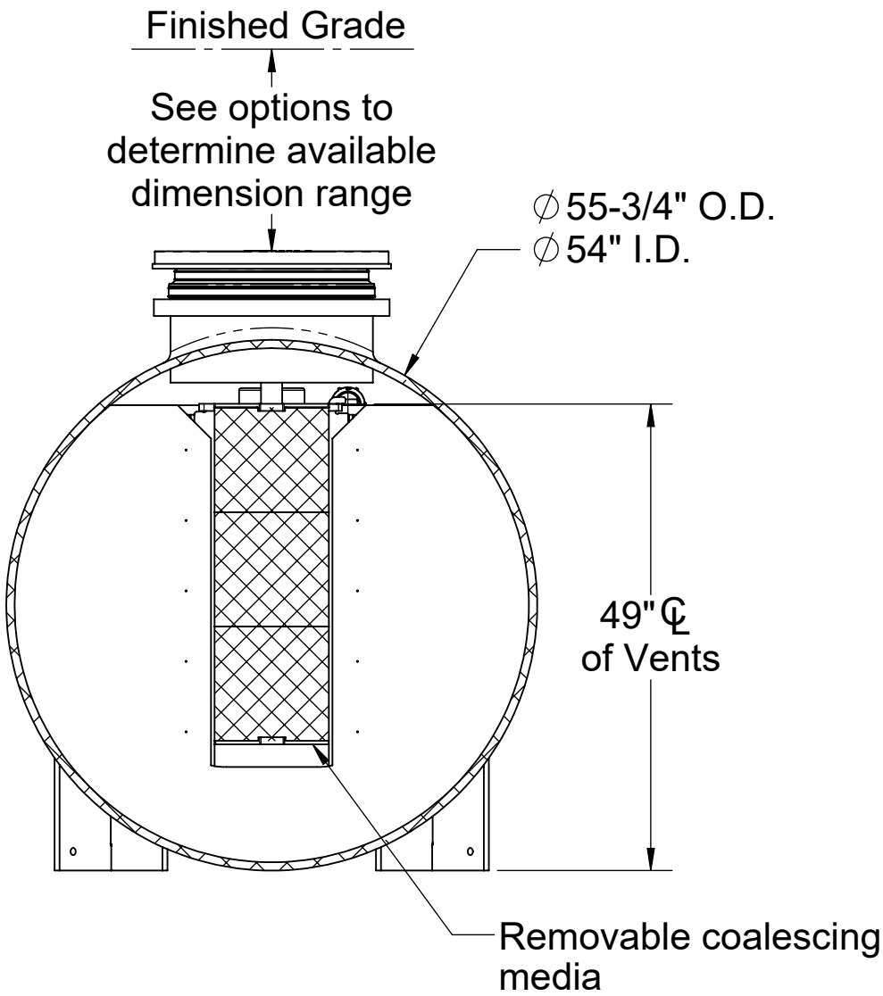
SECTION B-B
