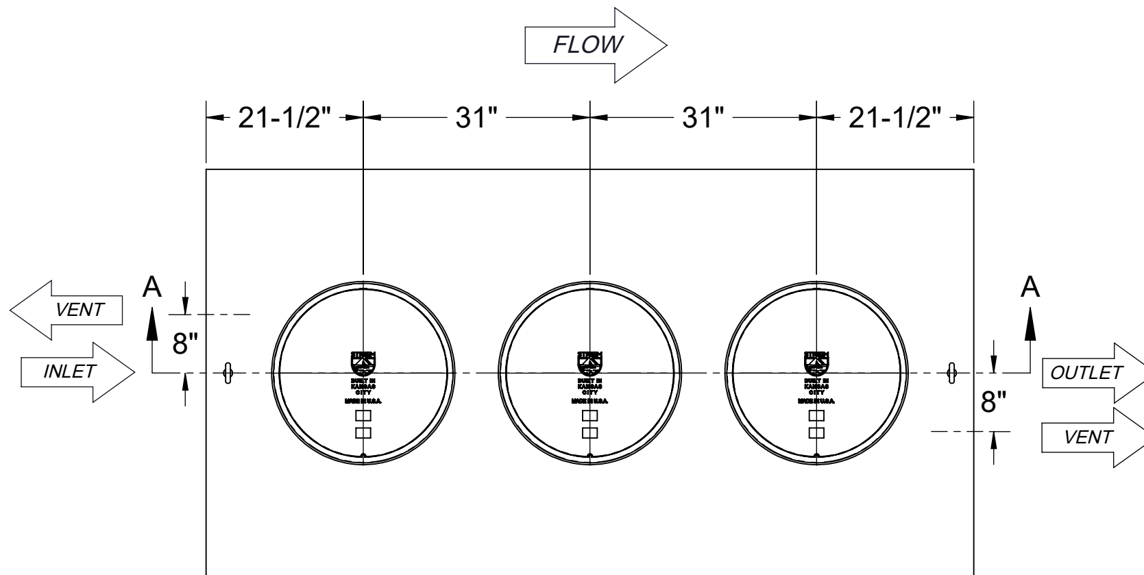
TOP VIEW
