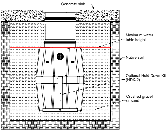
EXCAVATION AND BACKFILL DETAIL (INTERIOR OR EXTERIOR)
