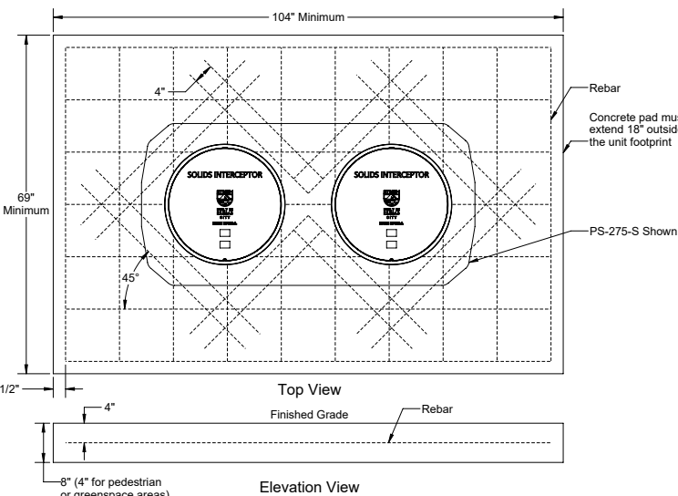
CONCRETE SLAB DETAIL FOR TRAFFIC LOADING
