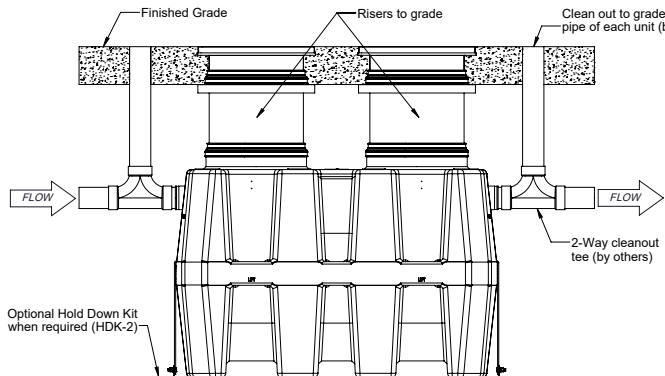
SIDE VIEW DETAIL
