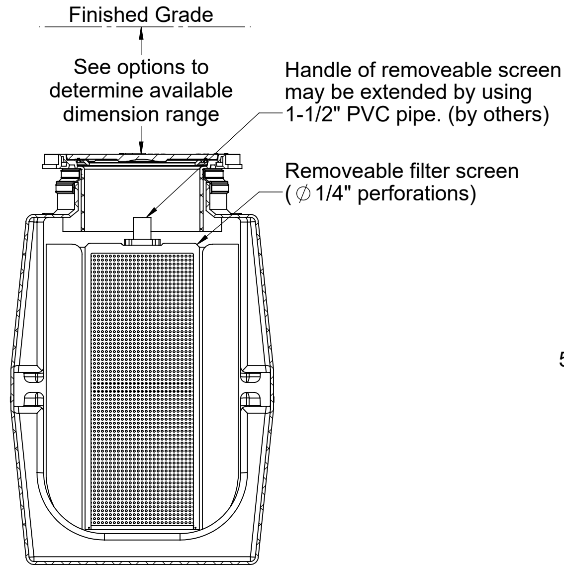
SECTION B-B
