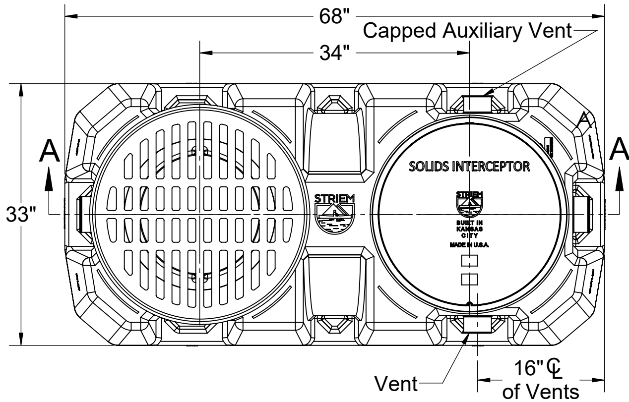
TOP VIEW
