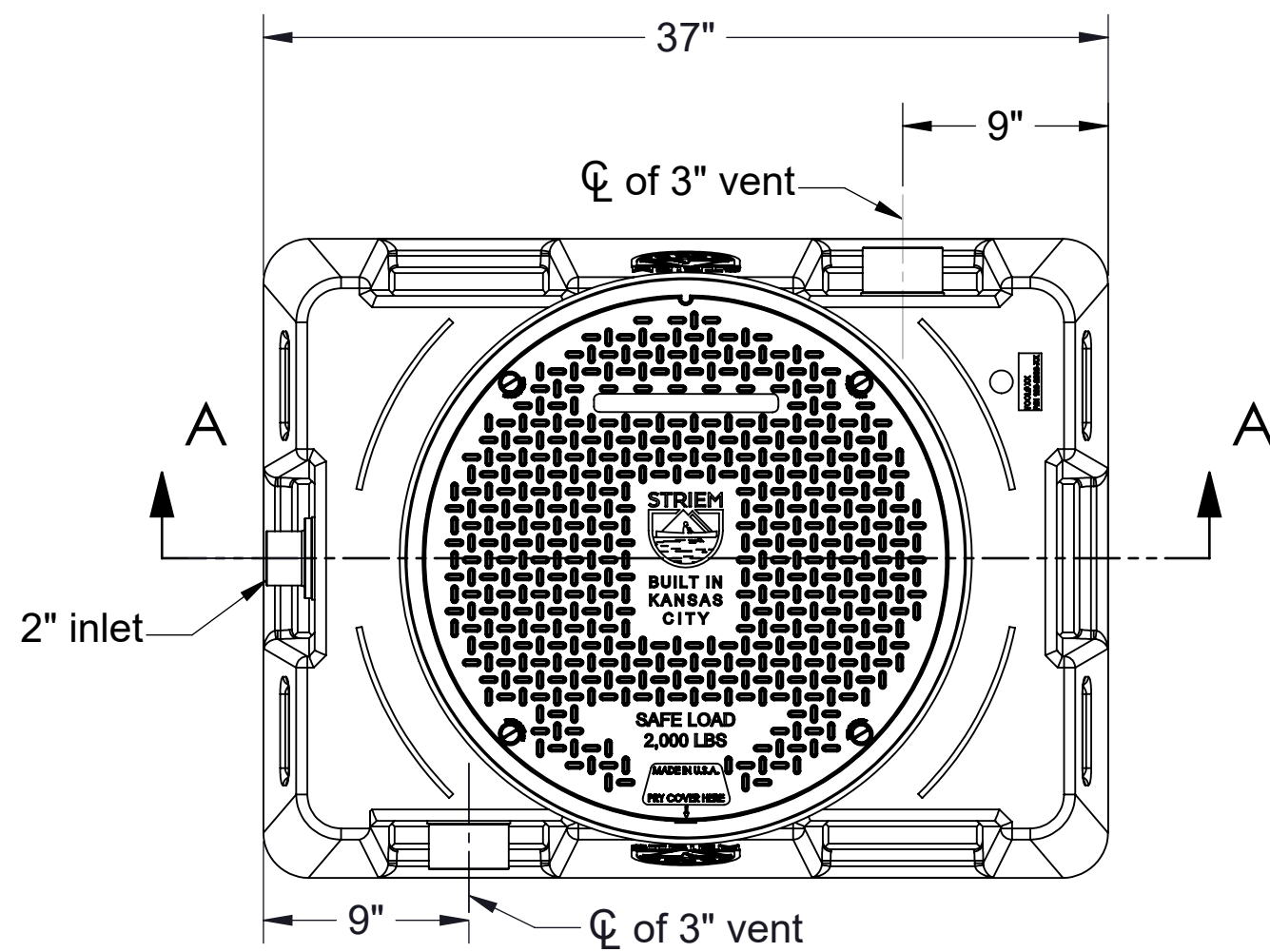
TOP VIEW
