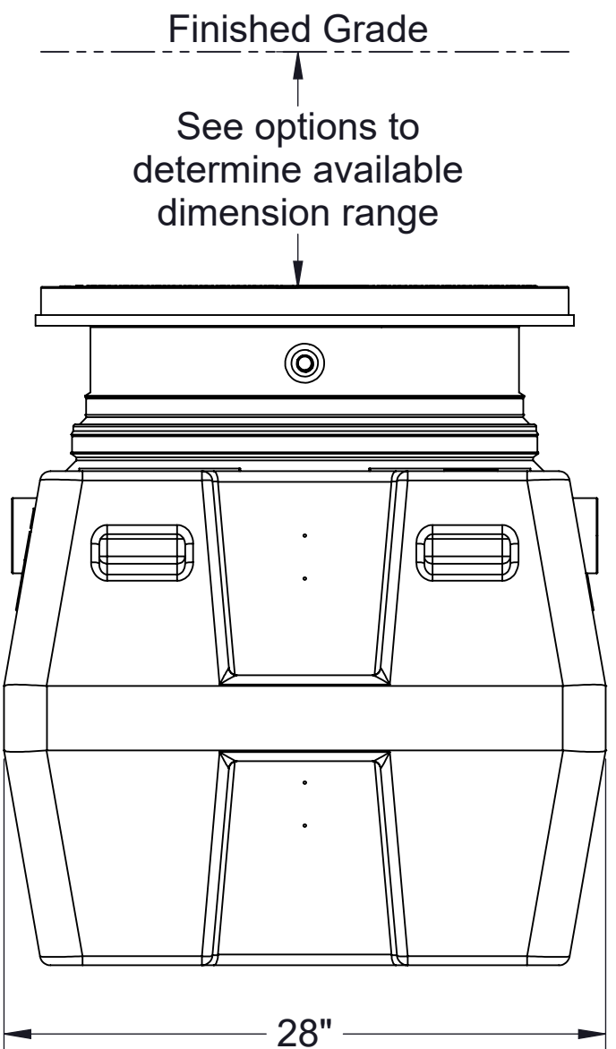
END VIEW
