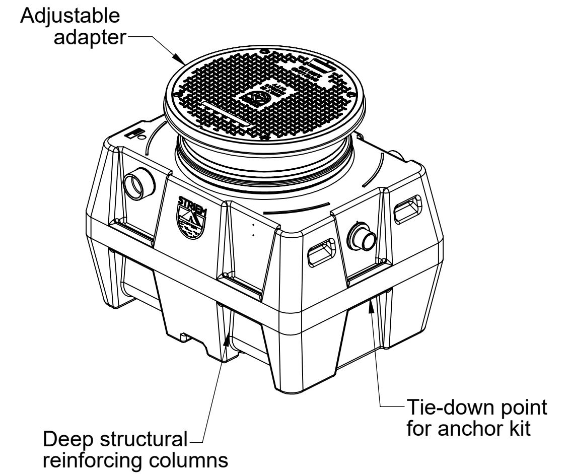
ISOMETRIC VIEW
