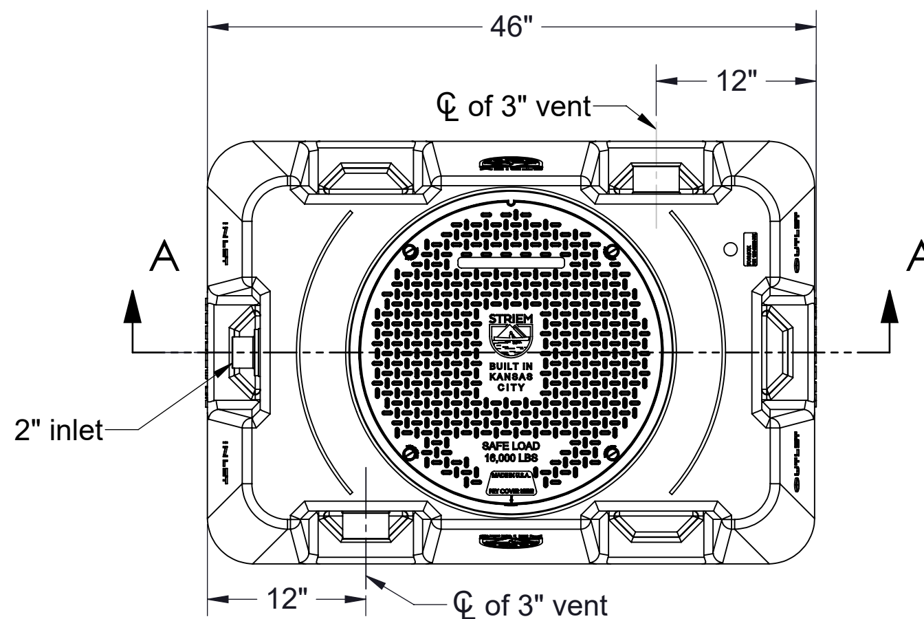
TOP VIEW
