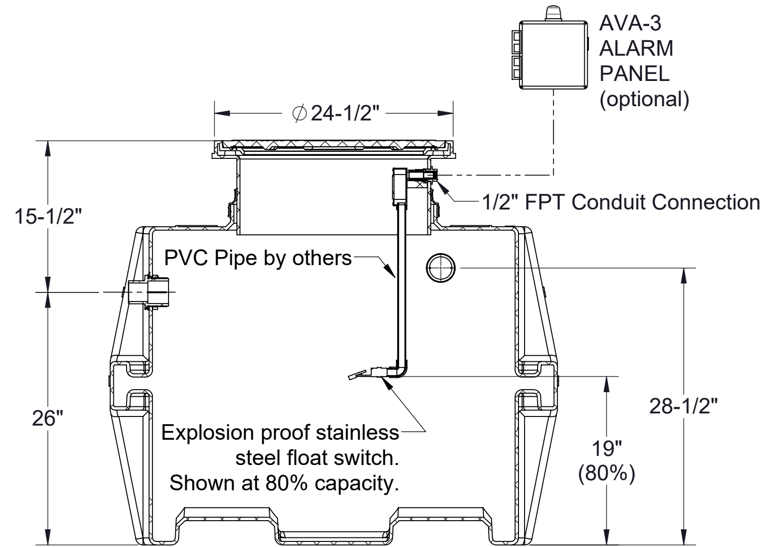
SECTION "A-A"
