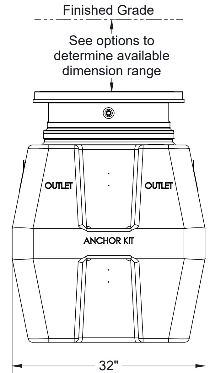
END VIEW
