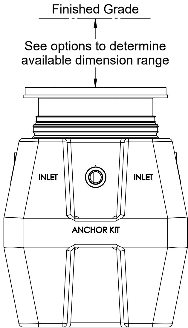
END VIEW
