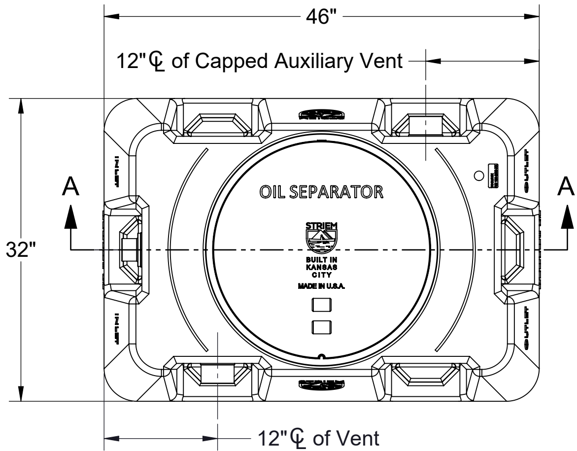
TOP VIEW
