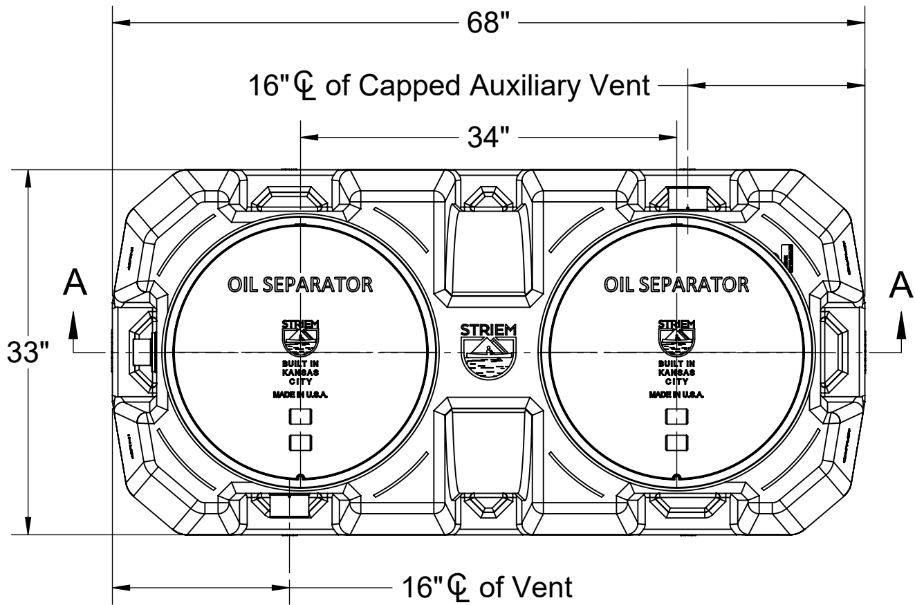
TOP VIEW
